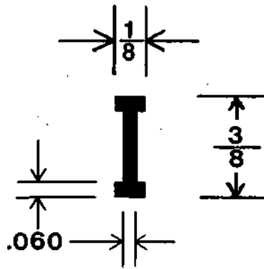
I-beam dimensions.
